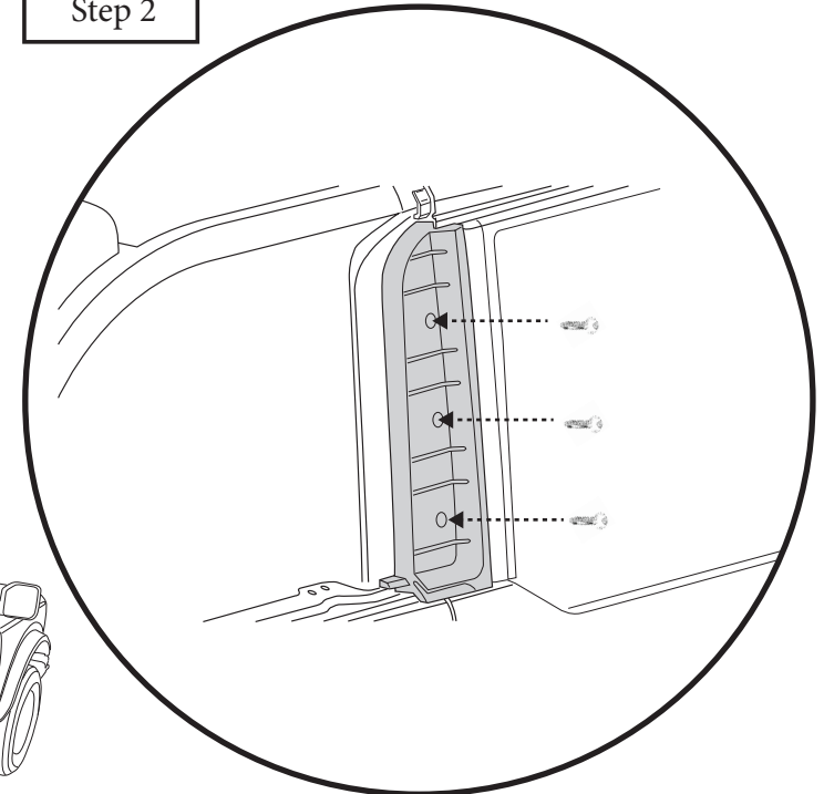
SCREW, M6 X 1.0 X 30mm Part #533.19 Qty. 6 T-30 Torx
