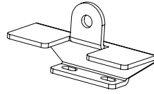
Sunrider Pivot Bracket #545.74 Qty. 2
