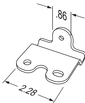
#2 Bow Pivot Bracket Part #579.95 Qty. 2
