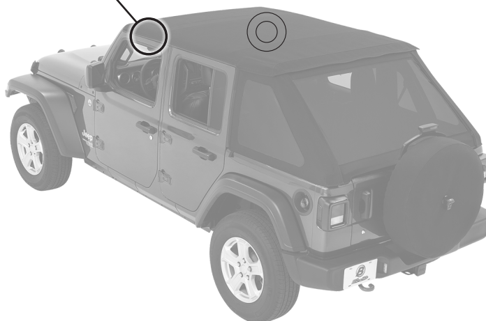
#2 Bow Link Assembly Part #576.15 - Left Qty. 1
