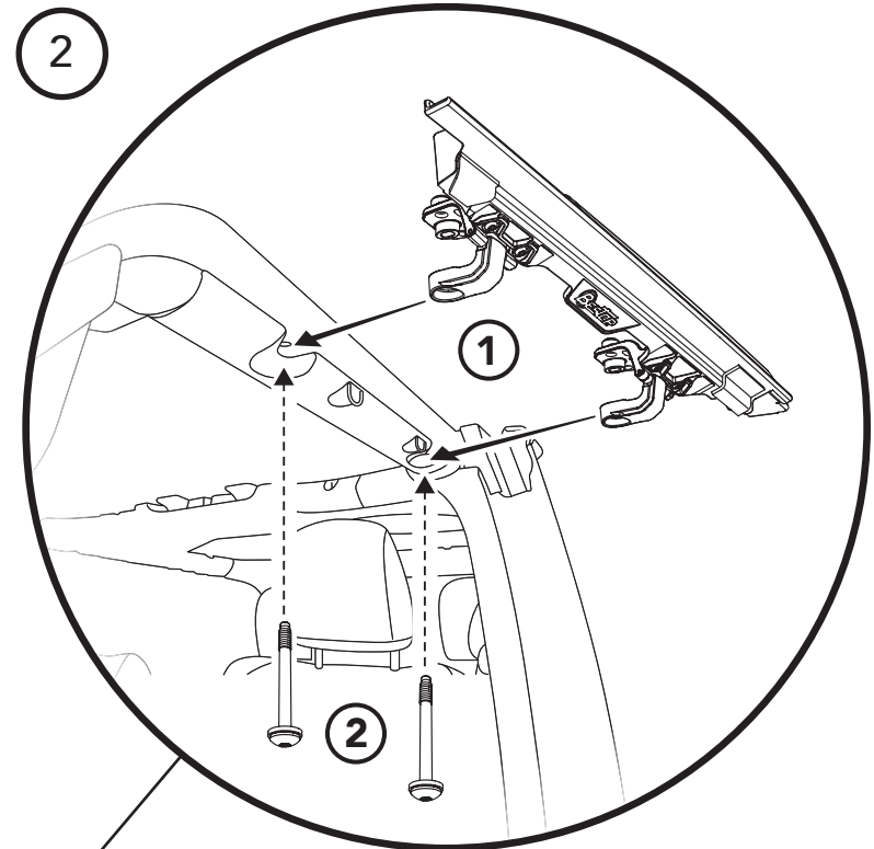
M8x1.25x20 Screw #573.09 Qty. 2
